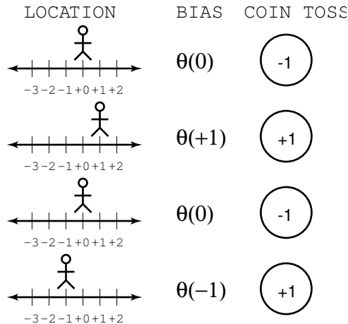
Figure 1: A walker performing his coin flips. We only see the right-hand column, but would like to recover the center column!
