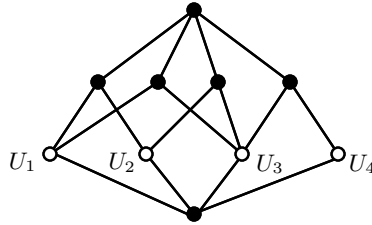
FIGURE 1. The intersection lattice of \mathcal{A} in Example 4.2
