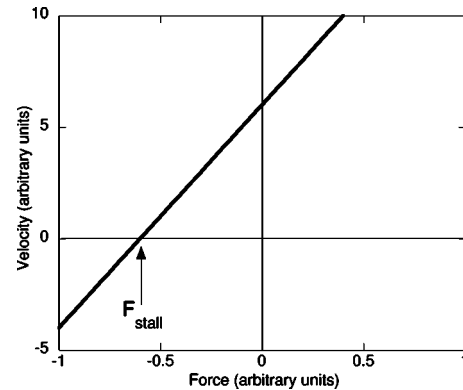
FIG. 2. Cartoon of a typical load-velocity curve of a Brownian motor in the presence of a load force. Without load force, the motor has a positive average velocity, while the motor moves backward when an excessive, negative force is applied. The stall force is the (negative) force at which the motor has zero velocity on average. Note that details of the force-velocity curve can look quite different from the cartoon shown here, including nonlinear behavior. In general, the motor velocity in response to a positive force can even be negative (negative absolute mobility 28-30 ).
