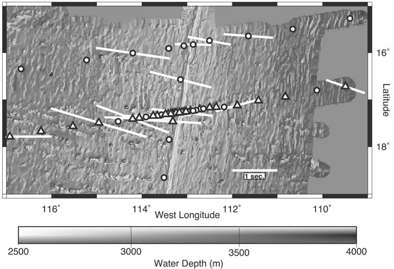
Figure 1. Bathymetric map of the southern East Pacific Rise with the locations of ocean bottom seismometers (circles and triangles) deployed during the MELT experiment. Current analysis uses data from a subset of OBSs (triangles) deployed along the primary array. Shear wave splitting measurements of Wolfe and Solomon [1998] are indicated by solid black lines; orientation and length of line represents fast polarization direction and split time, respectively.
