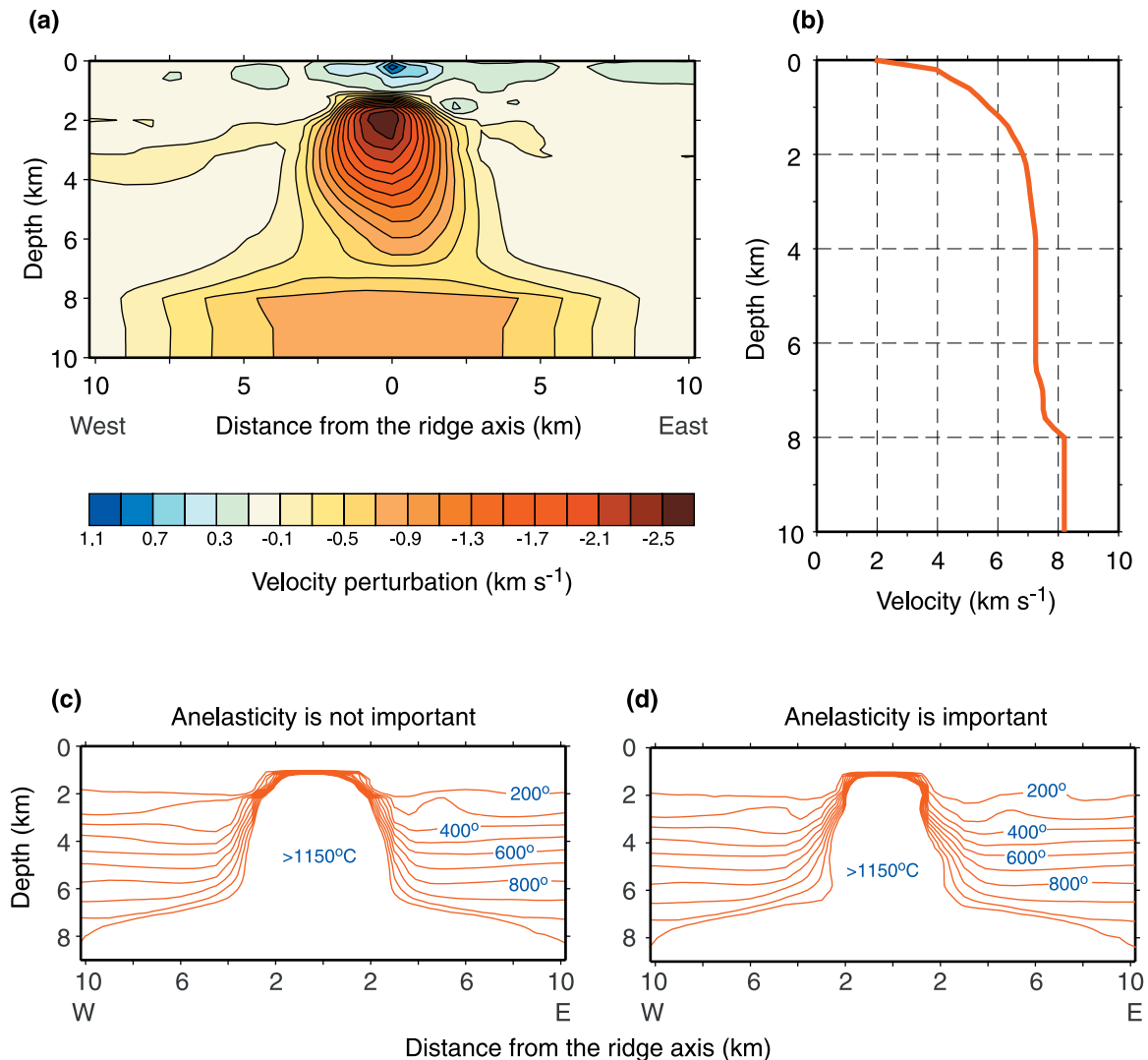
Figure 2. Velocity structure for a two-dimensional tomographic inversion on the East Pacific Rise at 9^{\circ}30'N and inferred temperatures (from Dunn et al. [2000]). Both (a) the velocity perturbations and (b) the one-dimensional reference velocity model are shown. The basic features of the velocity perturbation model are not strongly sensitive to the assumed crustal thickness. Models of the thermal structure were derived from the inversions assuming (c) anharmonic effects only and (d) both anharmonic and anelastic effects. These represent approximate minimum and maximum estimates of the contribution of temperature to the low velocity zone [ Dunn et al. , 2000]. Note that these thermal models assume a reference structure well off-axis with uniform vertical gradients, but that this is not required by the seismic data.
