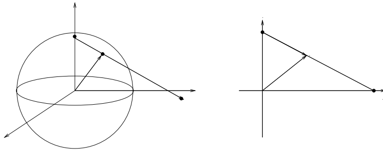
FIGURE 1. Stereographic projection
