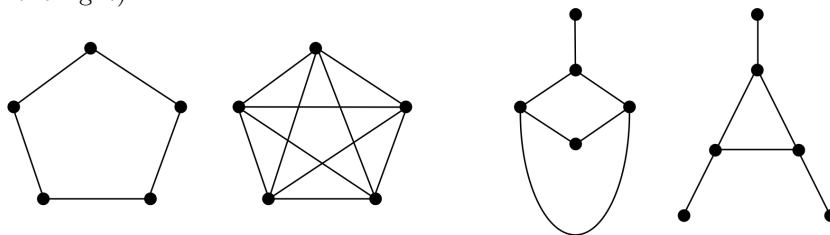
Fig. 11. Hamiltonian and not Hamiltonian graphs
