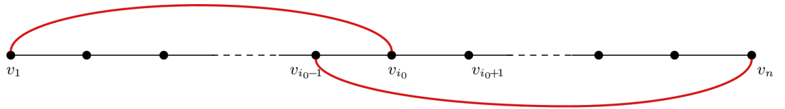
Fig. 13. A Hamiltonian cycle in G
